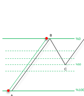
Fibonacci Retracment
