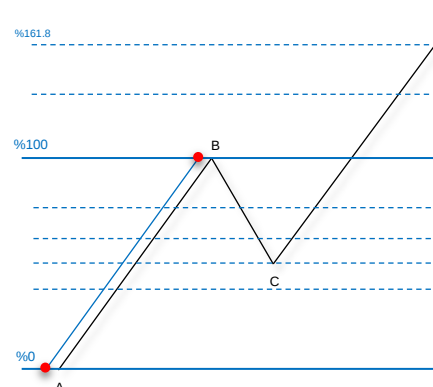
Fibonacci Extention
